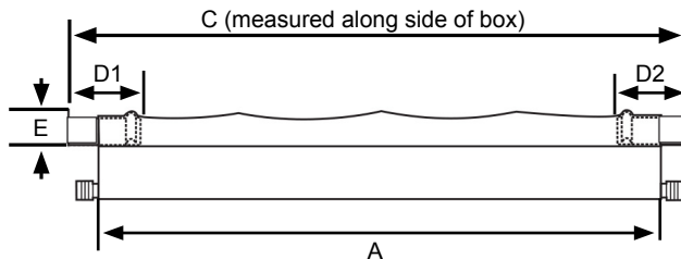
SIDE VIEW OF TARP SYSTEM
