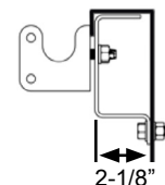
ILLUSTRATION 2 OFFSET BRACKET BASE
