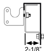
ILLUSTRATION 2 TARP STOP MOUNT SPACER BRACKET
